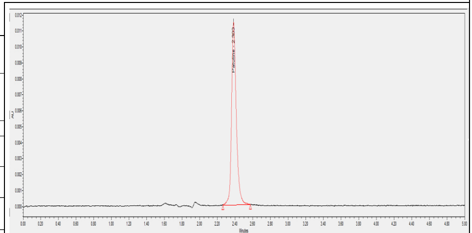
Chromatogram of Toxins
