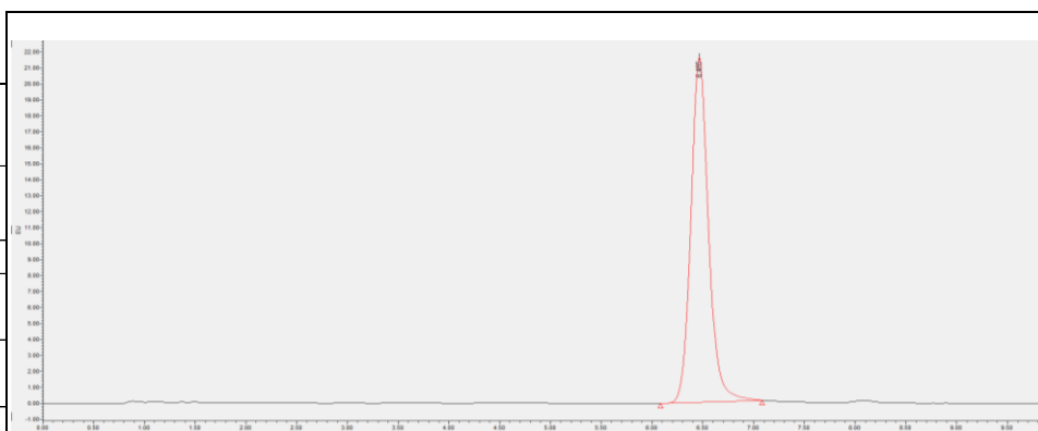
Chromatogram of Toxins
